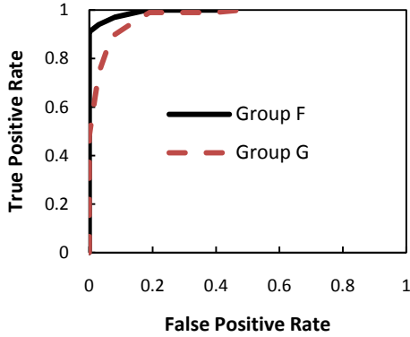
Figure 10: ROC curves of the uWave-based critical authentication
