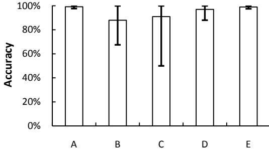
Figure 4: Recognition accuracy for non-critical authentication: range and average for Groups A to E
