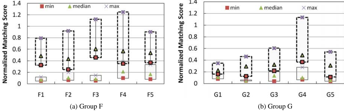
Figure 9: Matching distance of the owners (boxes with solid outlines) and the attackers (boxes with dashed outlines)
