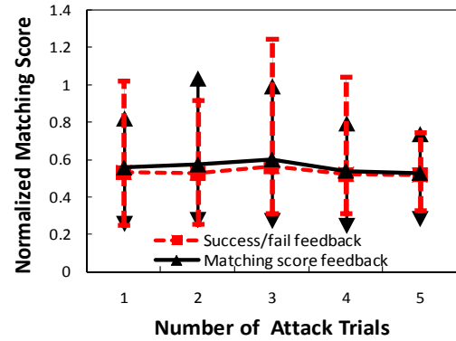
Figure 8: Normalized matching distances over multiple consecutive attack trials
