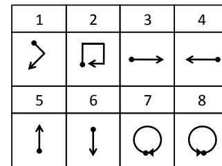
Figure 2: VTT gestures
