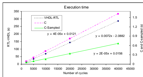
Fig. 8. Execution time for RTL-VHDL and our C-based power estimation
